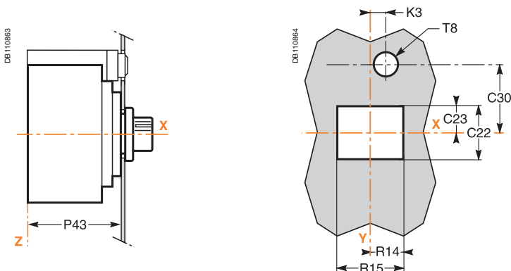
Dimensions (mm)
