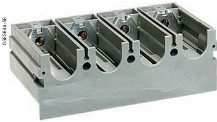
One-piece spreader.
