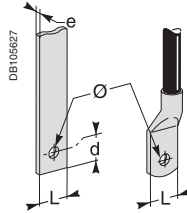
Connection of bars or cables with lugs.
