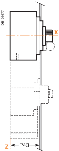
Direct handle (INS250/INV100 to 250)
