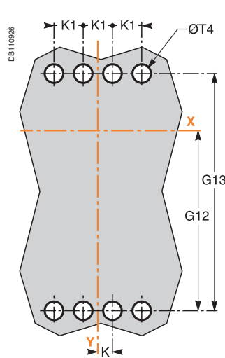
Fixed rear connection
