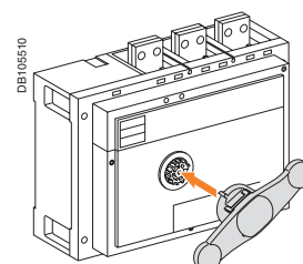
Direct rotary handle on INS/INV800 to 1600.
