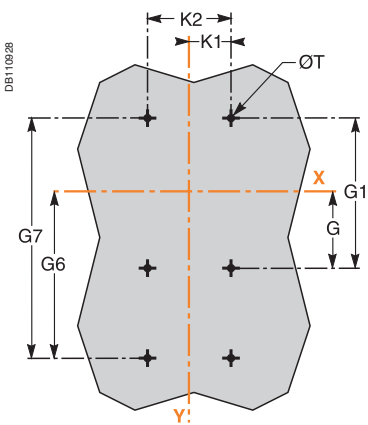
Fixed front connection
