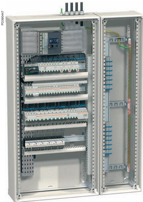
Power distribution incomer in a Prisma cubicle.
