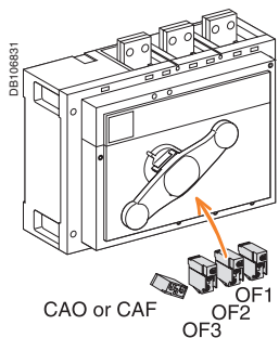
Interpact INS/INV800 to 1600.
