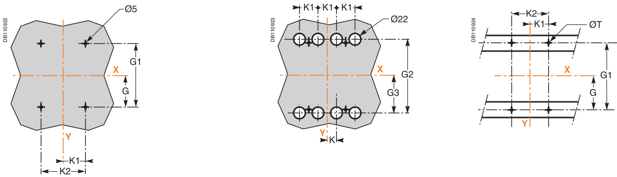
Dimensions (mm)
