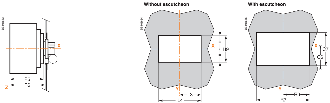
Dimensions (mm)
