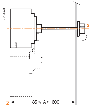
Extended handle
