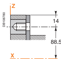
Small lugs for aluminium cables.
