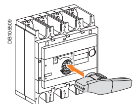
Direct rotary handle on INS/INV320 to 630.
