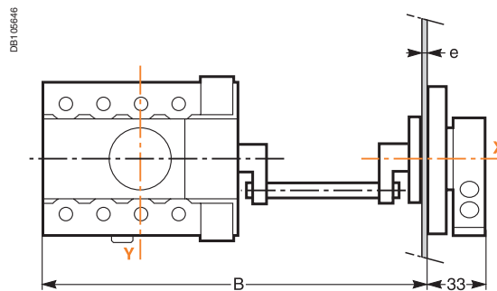
Dimensions (mm)
