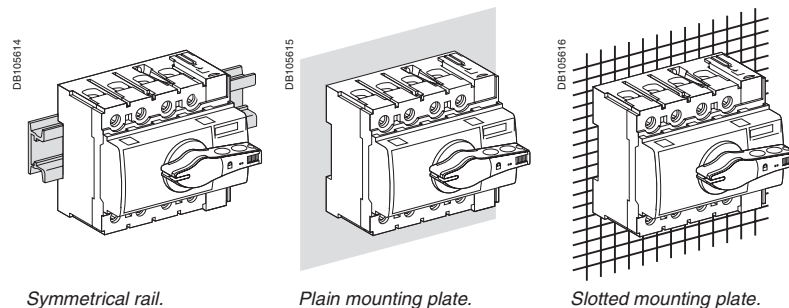
Symmetrical rail.
