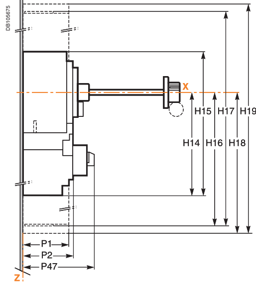
Extended handle
