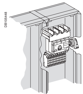
Installation in a 300 mm duct.
