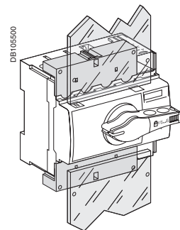
Terminal shrouds for Intercompact INS40 to 160 (with insulating plate to avoid contact with the conductors).
