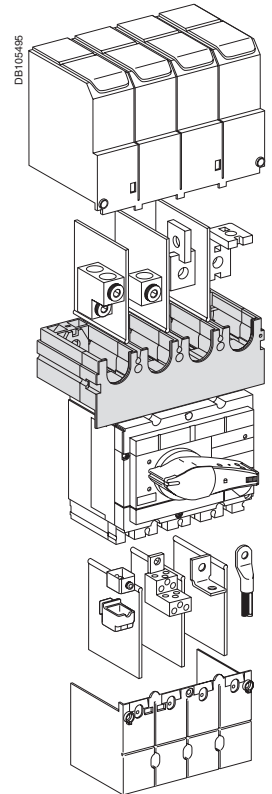
Connection and insulation accessories are identical to those for Compact NS.
