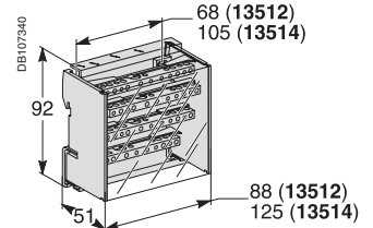
Multi-stage distribution block.
