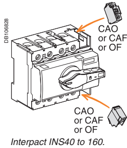
Interpact INS40 to 160.
