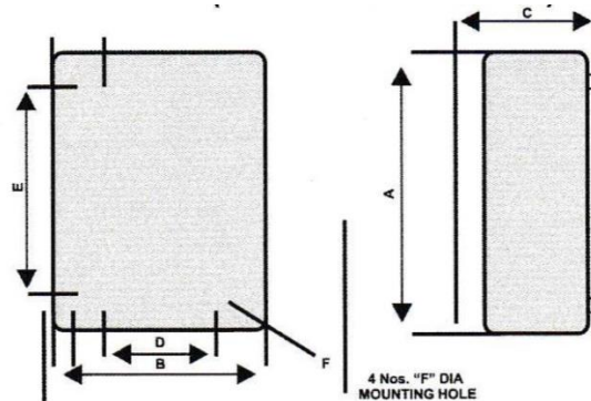
BUSBER (Copper/ Aluminium)
