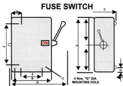
FUSE - SWITCH
